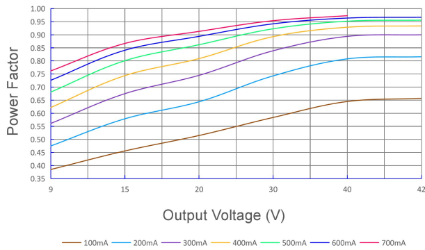
230Vac/50Hz Power Factor Vs Output Voltage(V)
