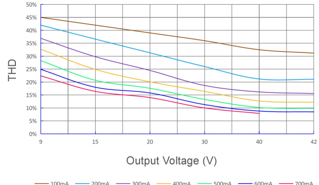
230Vac/50Hz THD Vs Output Voltage(V)
