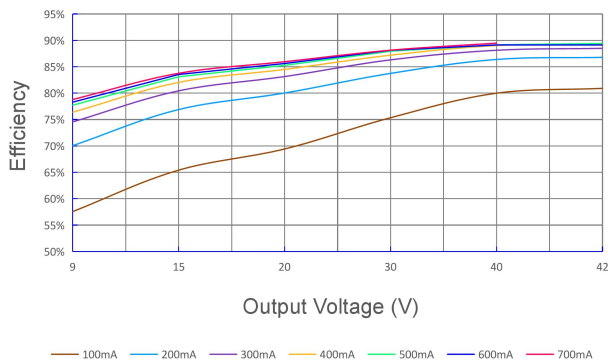
230Vac/50Hz Efficiency Vs Output Voltage(V)
