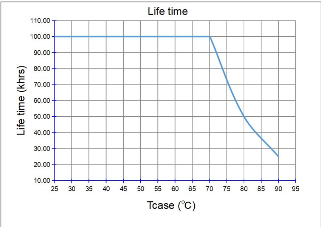
at Tc 80°C (0.2% / 1,000 h failure rate)
